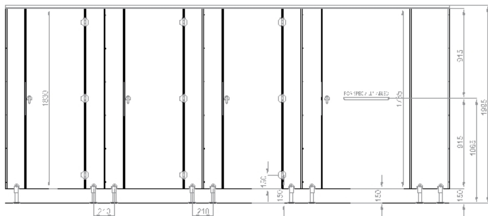
INTERIOR ELEVATION
