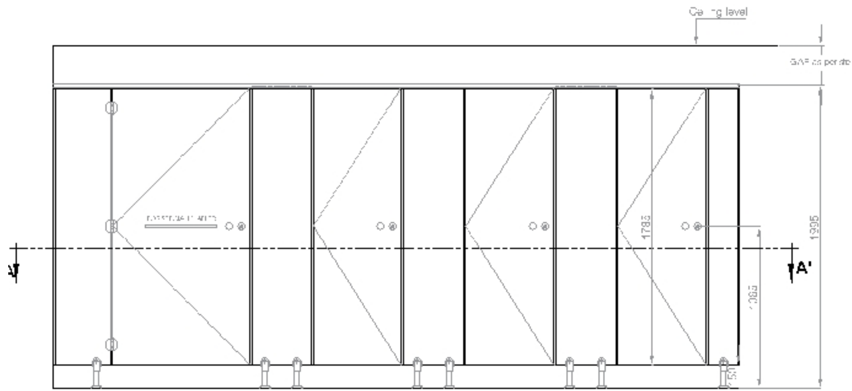
EXTERIOR ELEVATION
